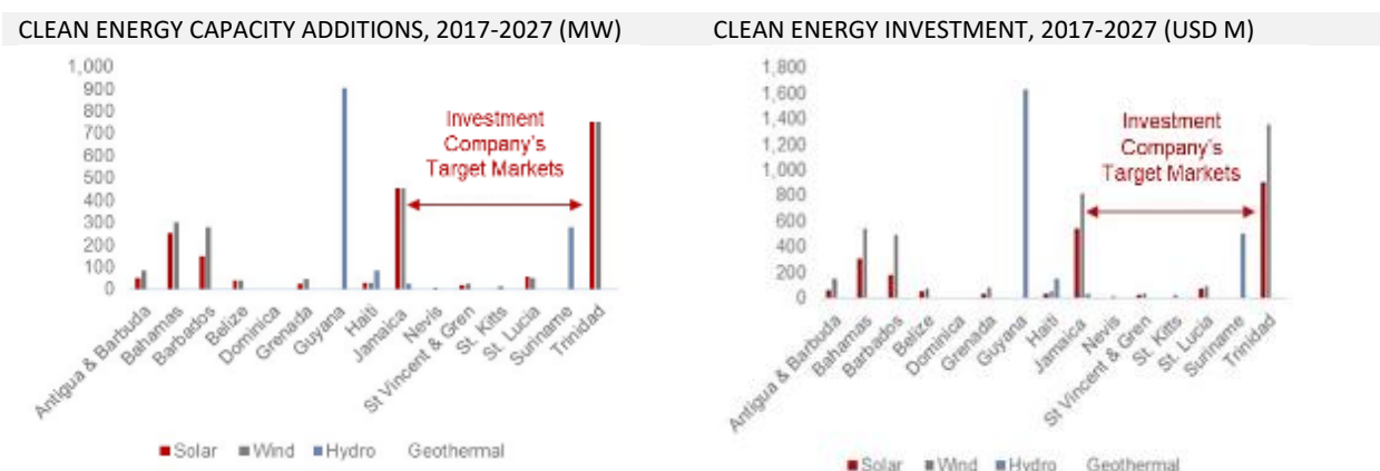
Chart 11.5 - CARICOM clean energy investment targets to 2027 16
